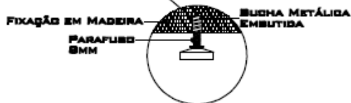
VISTA FRONTAL
